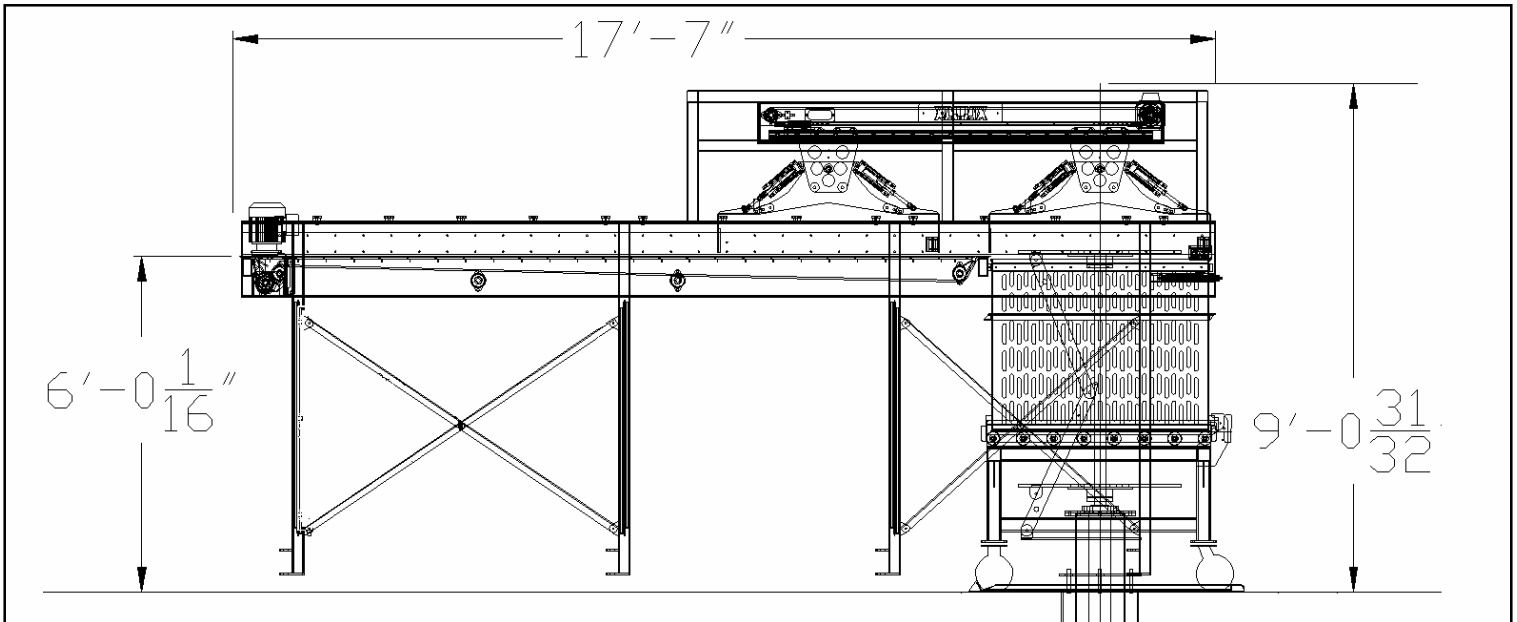
300X Series General Arrangement
