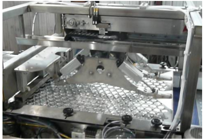
Servo Controlled Sweep Head and VFD controlled product conveyor.
